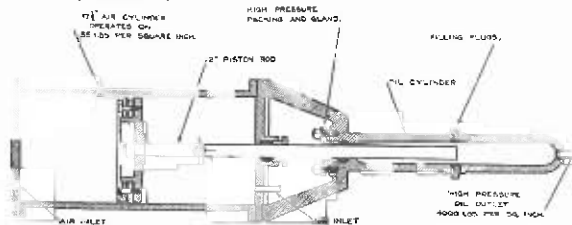
CROSS SECTION OF HIGH PRESSURE OIL GENERATOR FOR BRACE LOCKS JORDAN TYPE "A" SPREADER-DITCHERS
