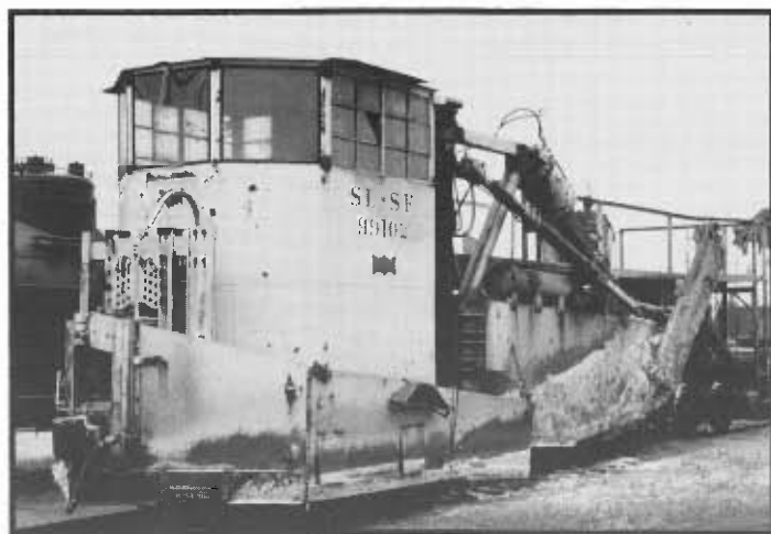
Frisco Jordan Spreader-Ditcher #99102, Sherman, TX, April, 1974. E. Stoll photo
