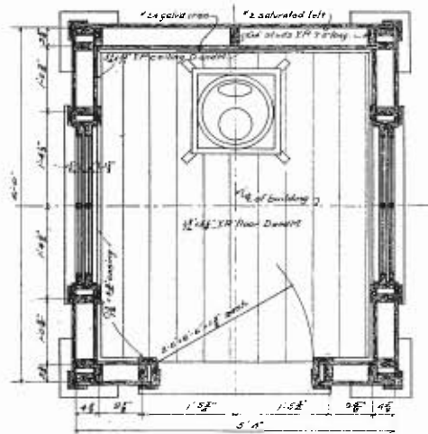
FLOOR PLAN
